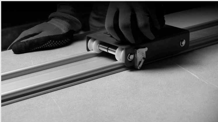
CUTTING DETAIL WITH GUIDE ON SLAB
